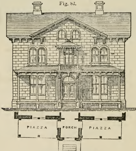
FRONT ELEVATION—No. 2.
